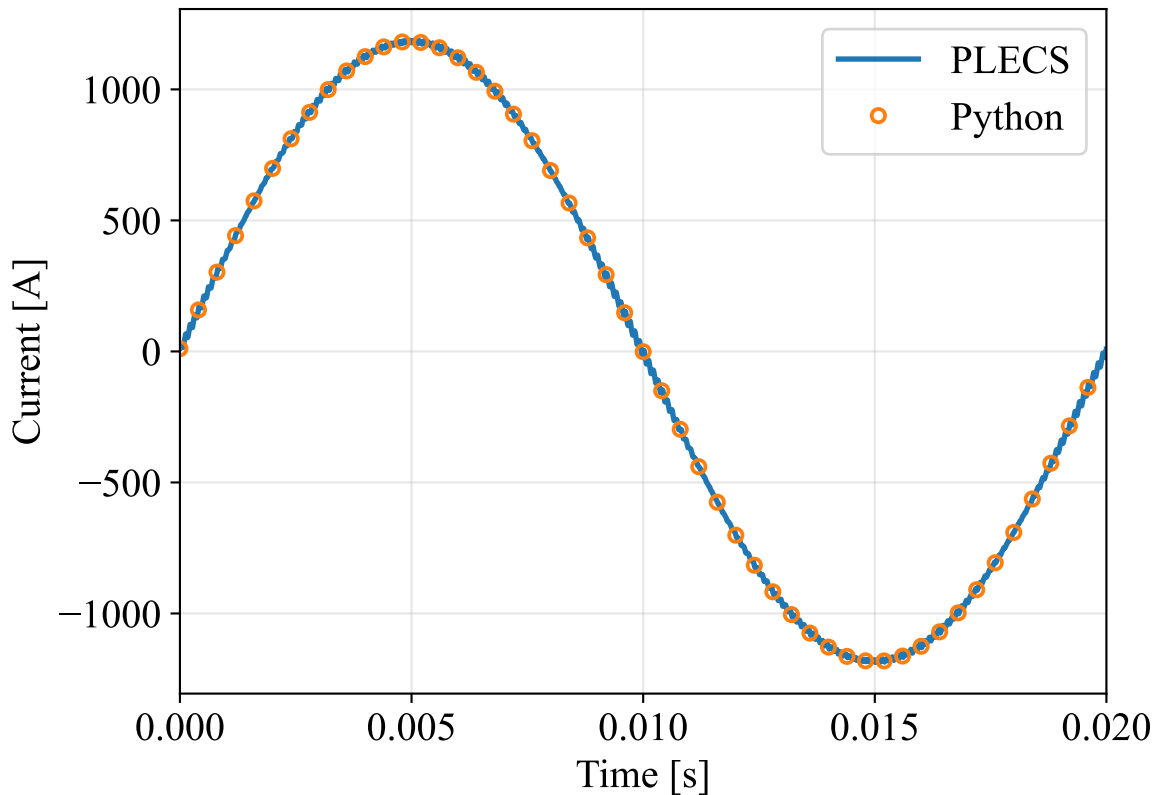
Grid-side current.
